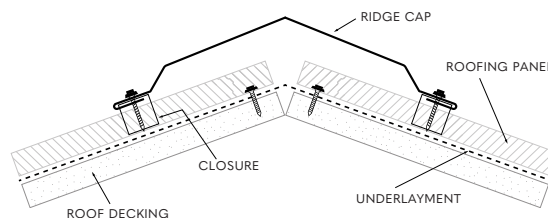
RIDGE CAP
