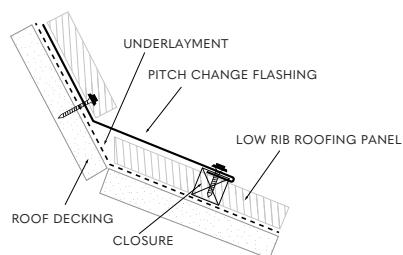
PITCH CHANGE
