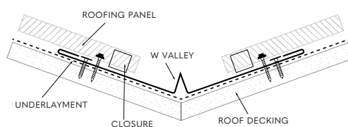
VALLEY
