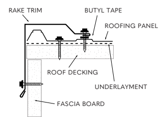
RAKE & GABLE
